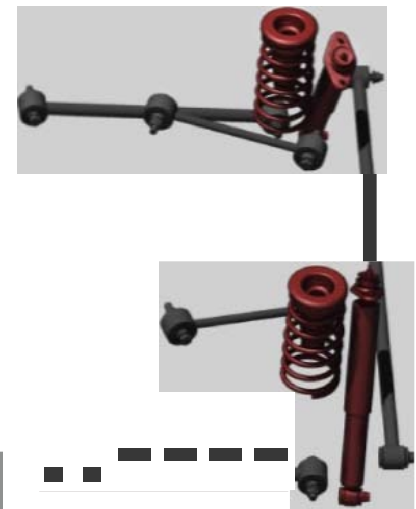
5 Link Rear Suspension
